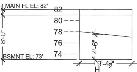
BSMNT WALL COVERAGE DIAGRAMS
